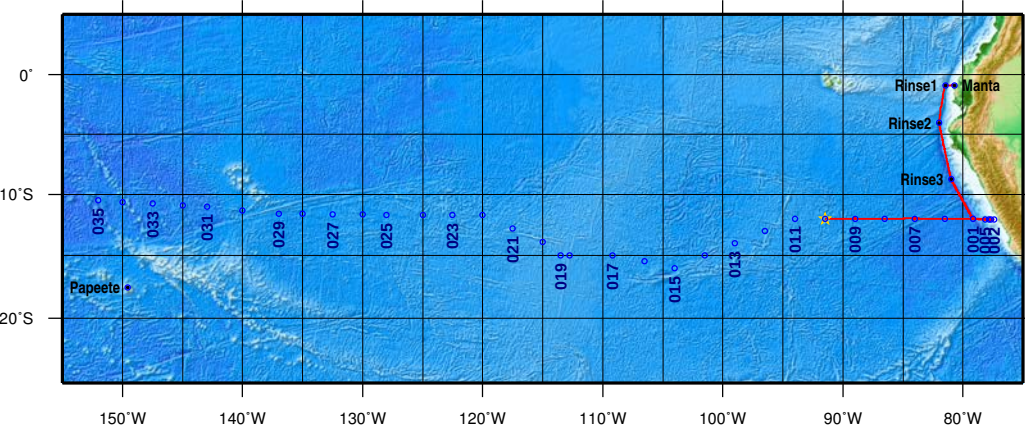
GEOTRACES-EPZT Cruise Track 2013-11-10 06:03 UTC
